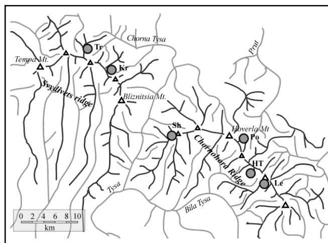
Fig. 1. Map of sampled populations of G.lutea in the Ukrainian Carpathians (represented by grayed circles). Kr – polynyna (mountain grassland) Krachuneska; Tr – the ridge slope between Troyaska and Tataruka Mountains; Sh – Sheshul and Pavlyk Mts.; Po – Pozhizhevska Mt.; HT – Hutyn Tomnatek Mt.; Le – polynyna Lemska.
